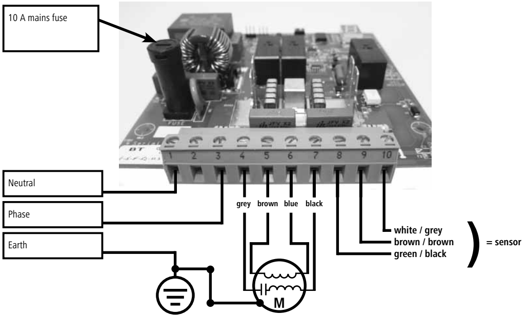
Figure 5.2: Wiring diagram for CowCleaner Swing up to 2015
