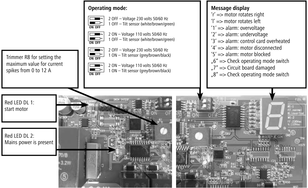
Figure 4.2: Circuit board for CowCleaner Swing up to 2015
