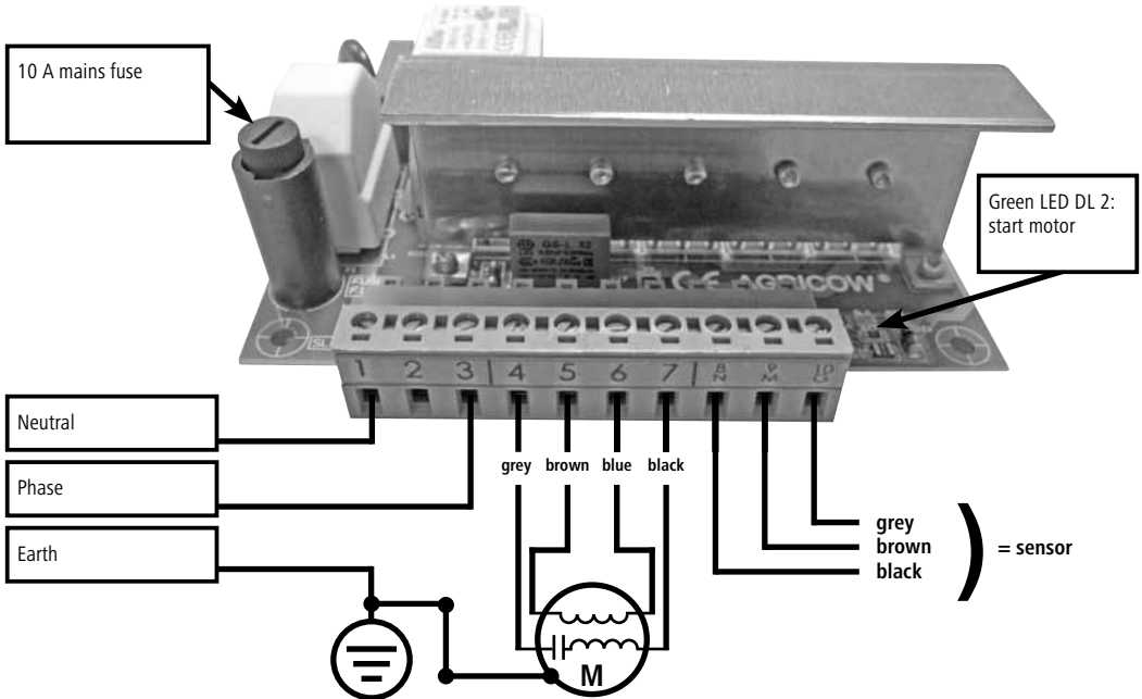
Figure 5.2: Wiring diagram for CowCleaner Swing up to 2015
