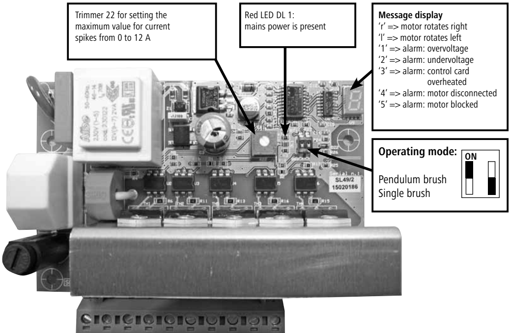
Figure 4.2: Circuit board for CowCleaner Swing up to 2015
